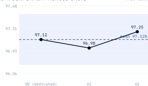
Figure 4. Purity conformity across tested units with mean and plus or minus 3 SD control band (SD 0.140%).
