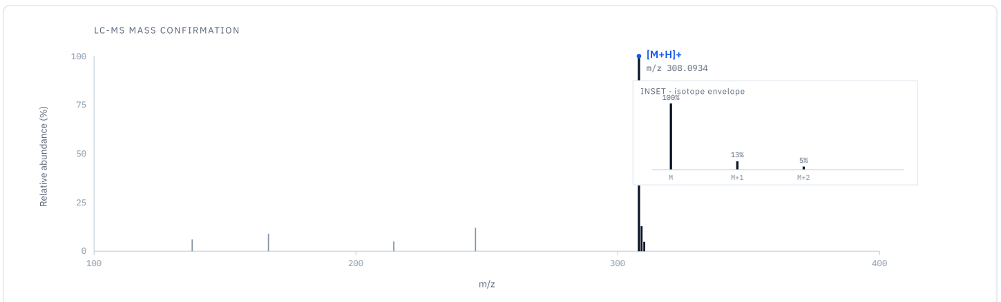
Figure 3. LC-MS mass confirmation (electrospray positive mode). Base peak [M+H] + at m/z 308.0934 matches glutathione (C10H17N3O6S, MW 307.32 Da); the isotopic envelope [M+1] (12.8%) and [M+2] (4.8%) confirms identity.
